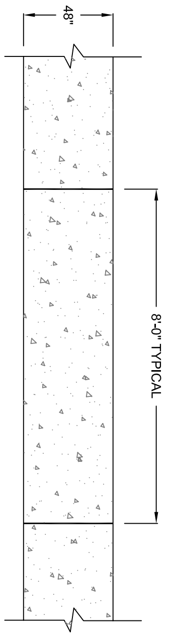
JOINT SPACING - PLAN VIEW NOT TO SCALE
